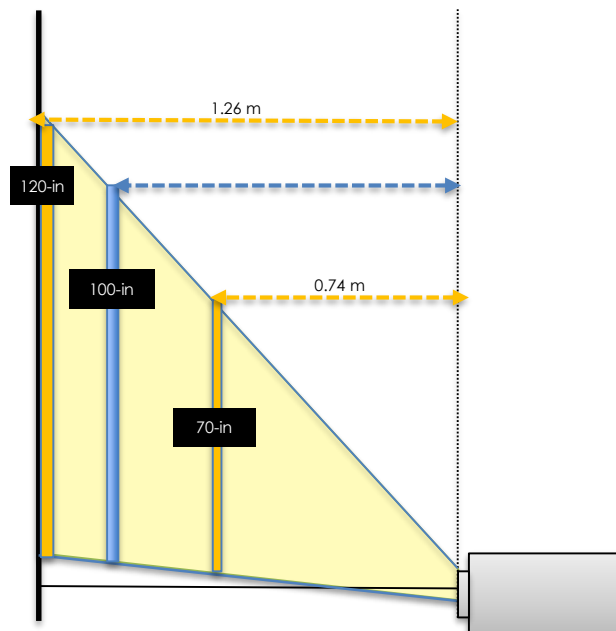
Optical axis when projected vertically against a screen
