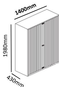
EUROTAMBOUR 4 tablettes H 1980mm L 1400mm P 430mm
